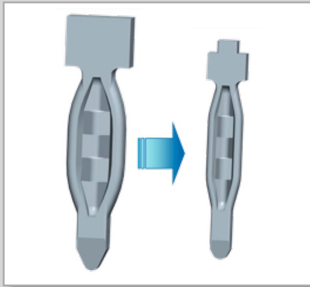
Picture 12 Standard Multispring and NanoMultispring pin.
